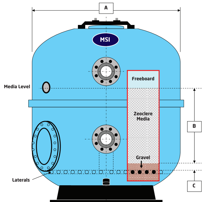
Based on: Lateral Under-drain - 1000mm bed depth
